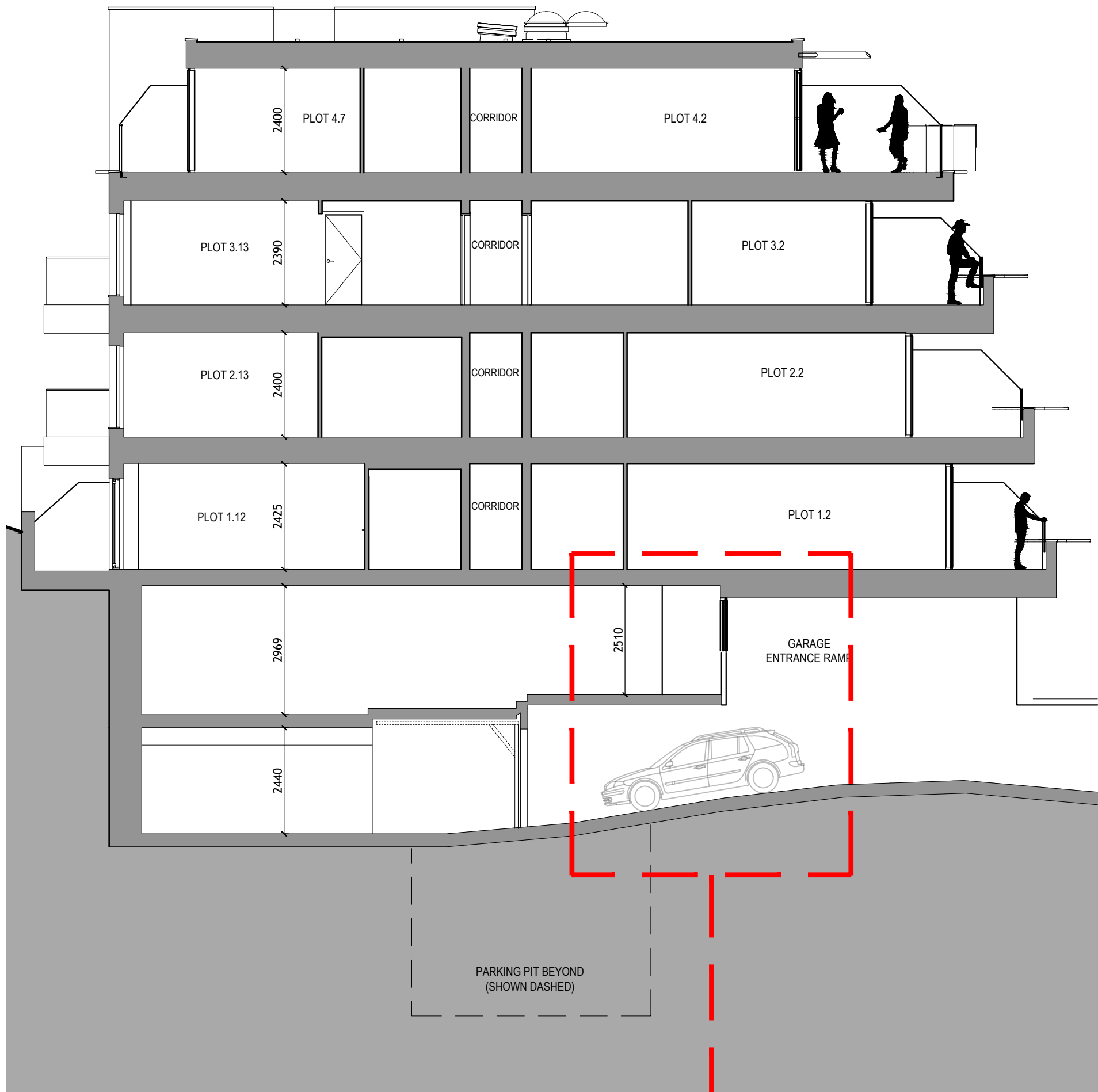
1 Section AA 1:100
