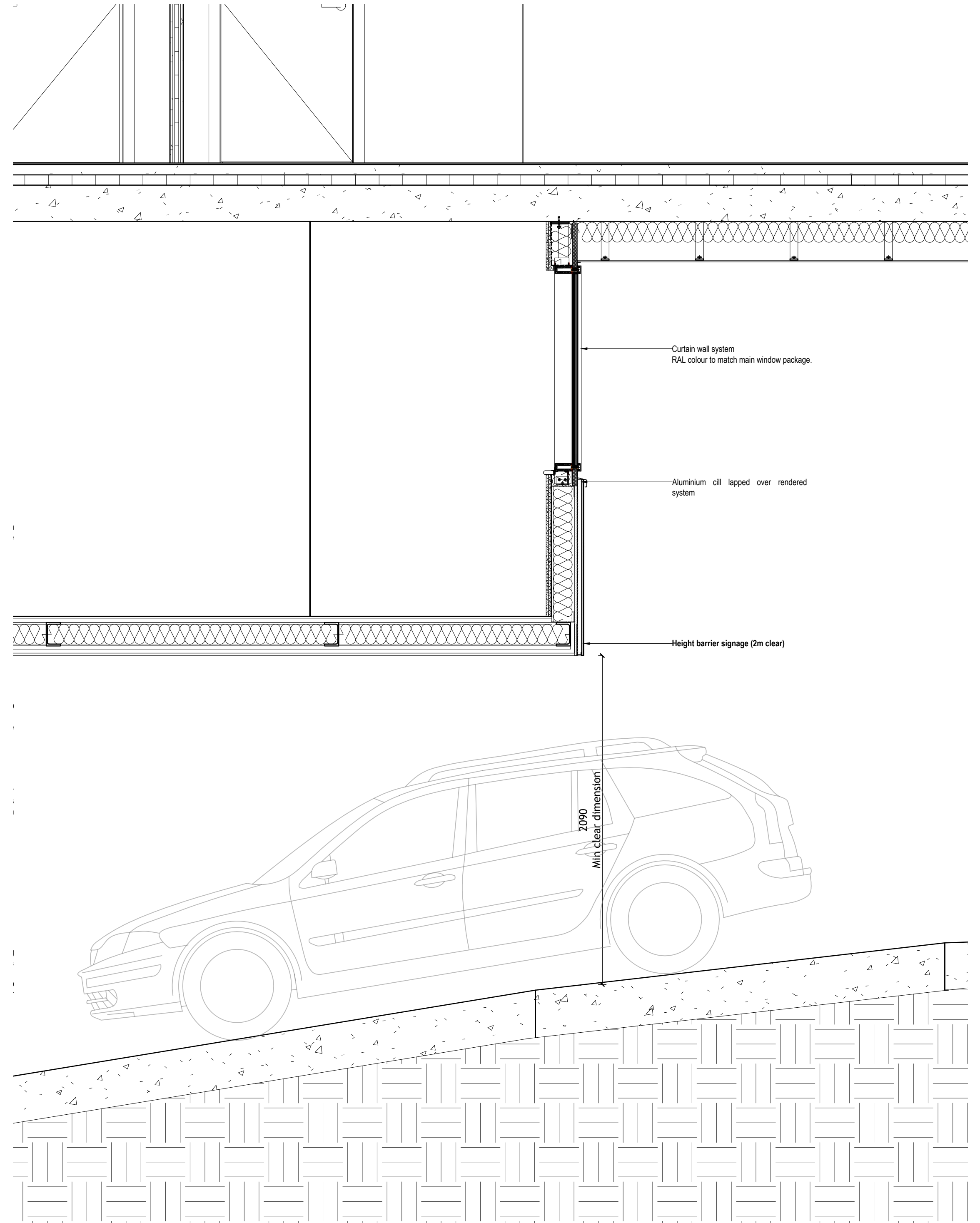
2 Section AA Through Drive Through - Mezzanine Link 1:20
